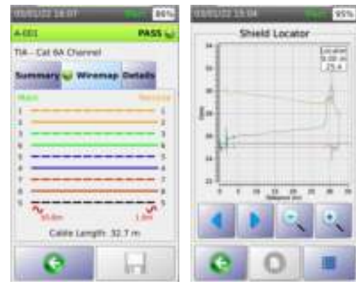
Fig 3 - Cable with AC shielding discontinuity and its time domain locator plot
